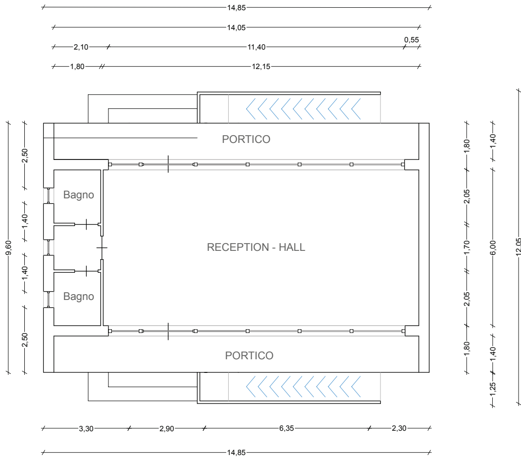
OSTELLO (RECEPTION- HALL) - Planimetria piano terreno
